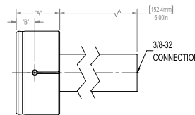
90.00 mm - 100.00 mm / 3.534 in - 3.937 in (2115008) Minimum recommended hole length: 6.35 mm / 0.250 in With guide sleeve or stop collar: 1.8 mm / 0.07 in
