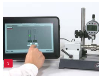
Radial run out measurement with dial indicator
