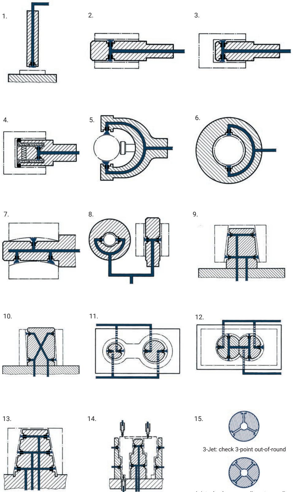
4-Jet: check average diameter readings which requires special amplifier
