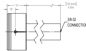
100.00 mm - 115.00 mm / 3.937 in - 4.528 in (2115009) Minimum recommended hole length: 6.35 mm / 0.250 in With guide sleeve or stop collar: 1.8 mm / 0.07 in
