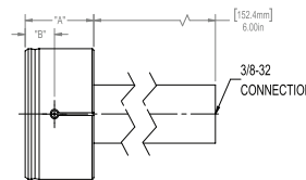
75.00 mm - 90.00 mm / 2.953 in - 3.534 in (2115007) Minimum recommended hole length: 6.35 mm / 0.250 in With guide sleeve or stop collar: 1.8 mm / 0.07 in
